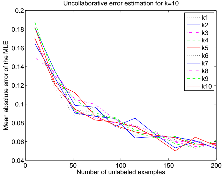
Figure 6: \text{mae}(\hat{\theta}^{\text{mle}}, \theta^{\text{true}}) as a function of n for each individual classifier k_i in Figure 4 (right). \theta_i^{\text{true}} = 0.75 \forall k_i and P(y = 1) = 0.75 . The estimation converges to the truth faster in the collaborative case (Figure 4 (right)) than in the non-collaborative case (this figure).
