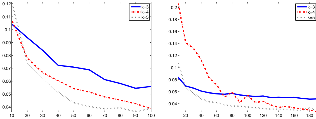
Figure 7: \text{mae}(\hat{\theta}^{\text{mle}}, \theta^{\text{true}}) as a function of n for different number of annotators k on RTE (left) and TEMP (right) datasets. Left: n = 100 , P(y = 1) = 0.5 and \theta^{\text{true}} = \{0.85, 0.92, 0.58, 0.5, 0.51\} . Right: n = 190 , P(y = 1) = 0.56 and \theta^{\text{true}} = \{0.93, 0.92, 0.54, 0.44, 0.92\} . The classifiers were added in the order specified.
