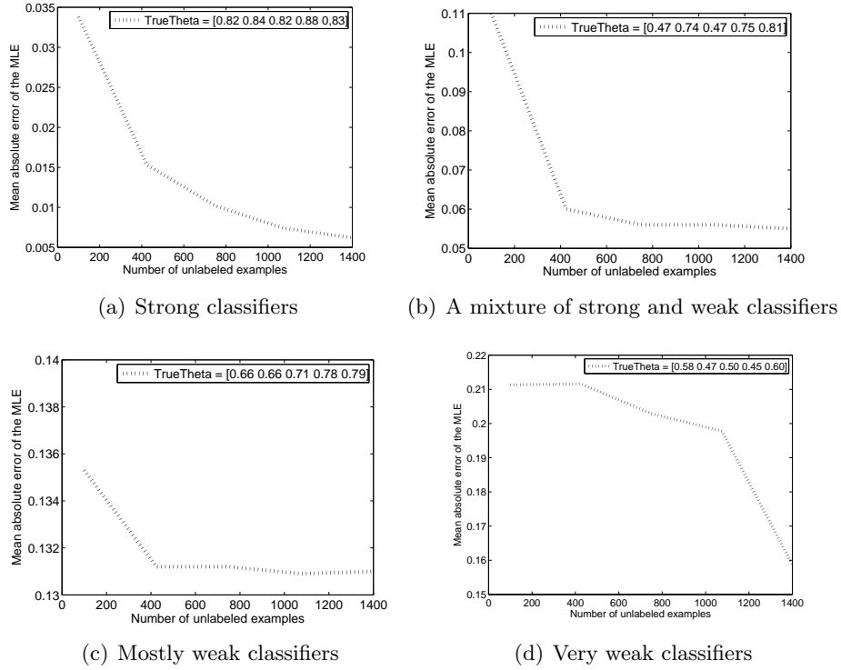
Figure 8: \text{mae}(\theta^{\text{true}}, \hat{\theta}^{\text{MLE}}) as a function of the test set size on the Ringnorm dataset. p(y = 1) = 0.47 , and \theta^{\text{true}} is indicated in the legend in each plot. The four panels represent mostly strong classifiers (upper left), a mixture of strong and weak classifiers (upper right), mostly weak classifiers (bottom left), and mostly very weak classifiers (bottom right). The figure shows that the framework is robust to occasional deviations from the assumption regarding better than random guess classification accuracy (upper right panel). However, as most of the classifiers become weak or very weak, the collaborative unsupervised estimation framework results in worse estimation error.
