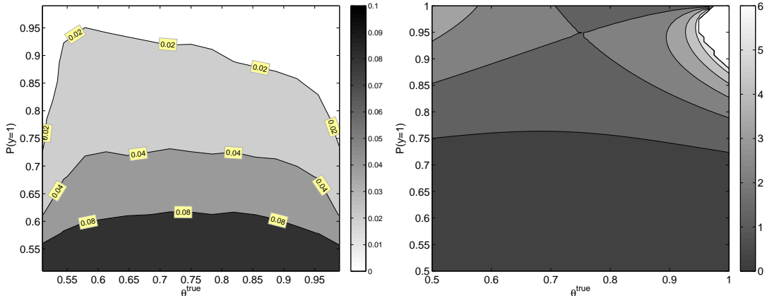
Figure 3: Left: Average value of |\hat{\theta}_n^{\text{mle}} - \theta^{\text{true}}| as a function of \theta^{\text{true}} and p(y = 1) for k = 1 classifier and n = 500 . The plot illustrates the increased accuracy obtained by a less uniform P(y) . Right: Fisher information J(\theta) for k = 1 as a function of \theta^{\text{true}} and P(y) . The asymptotic variance of the estimator is J^{-1}(\theta) which closely match the experimental result in the left panel.
